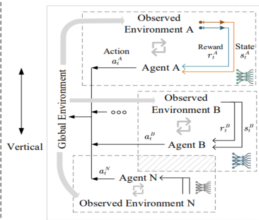
Vertical Federated Reinforcement Learning
