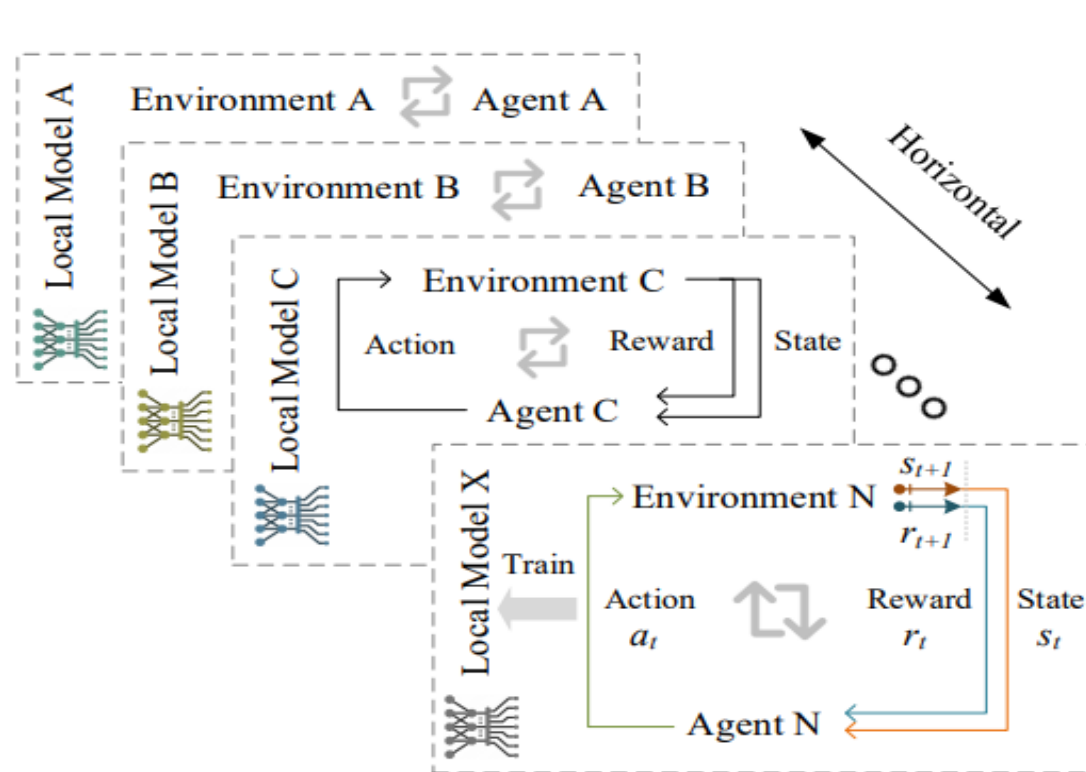
Horizontal Federated Reinforcement Learning
